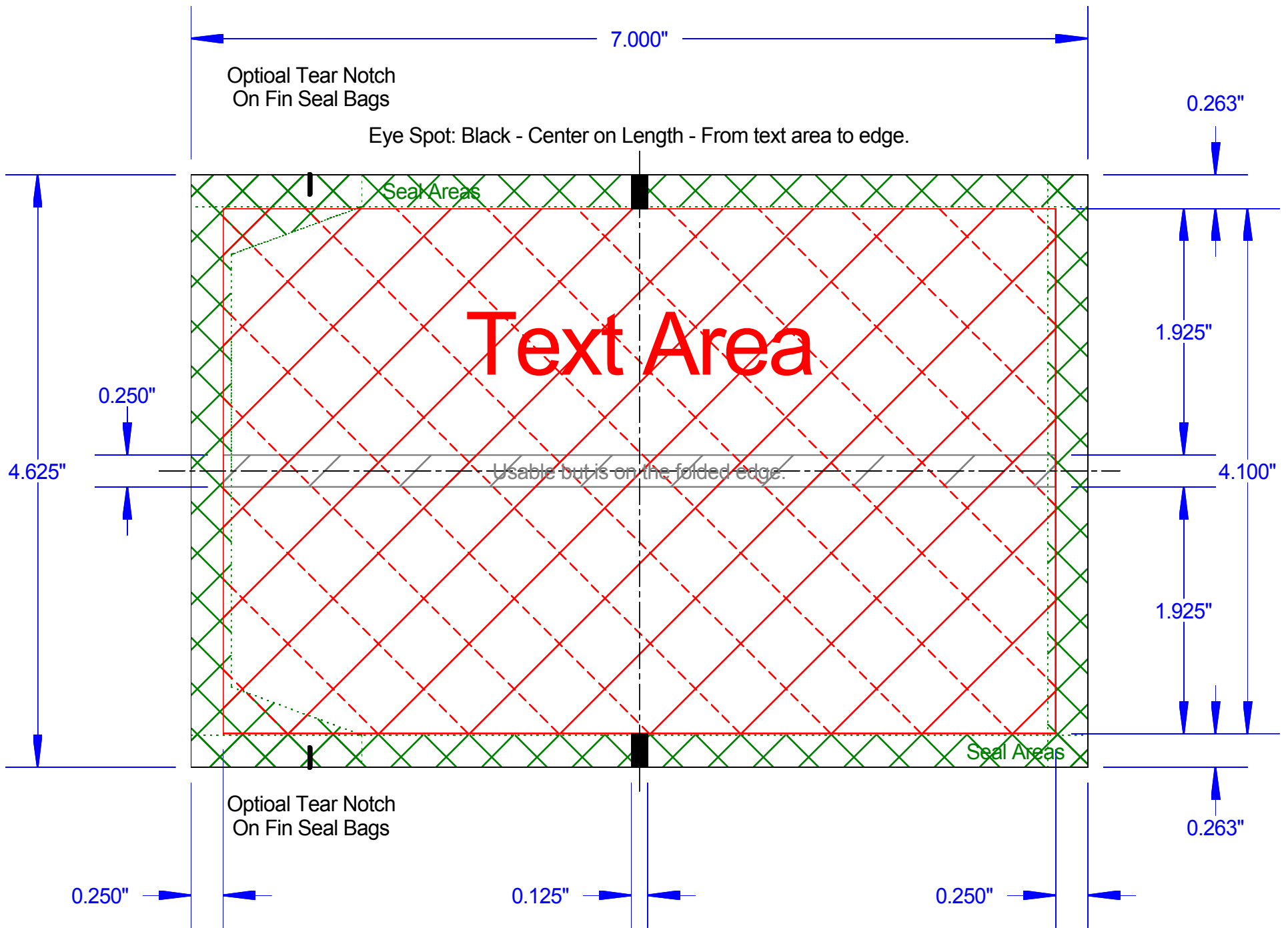
Barbie - DieLine 55mm former, Max bag size.
